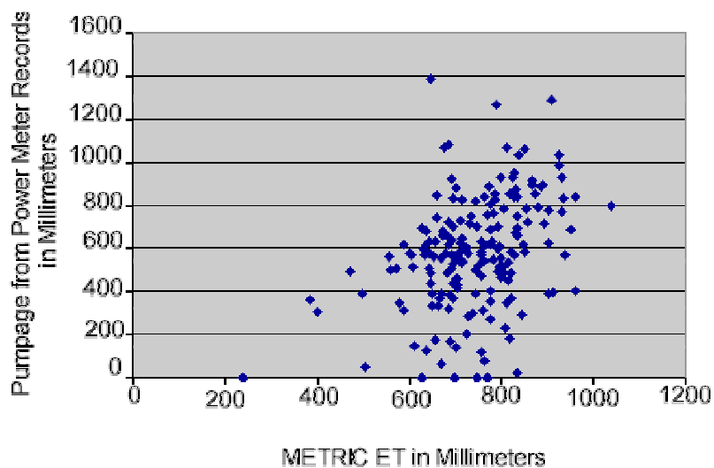
Figure 10. Ground-water pumpage from power consumption records versus METRIC ET in millimeters for the period April – October, 2000.
