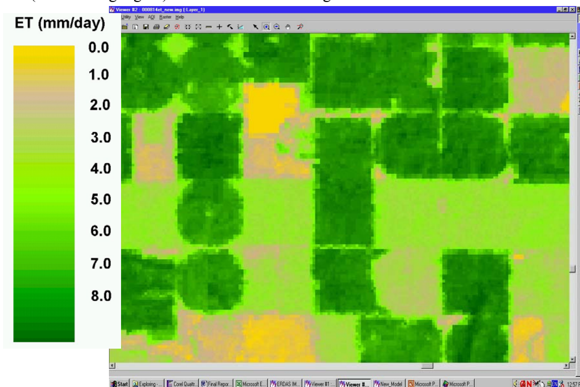
Figure 9. Closeup of evapotranspiration from individual irrigated fields in southern Idaho on August 14, 2000.
