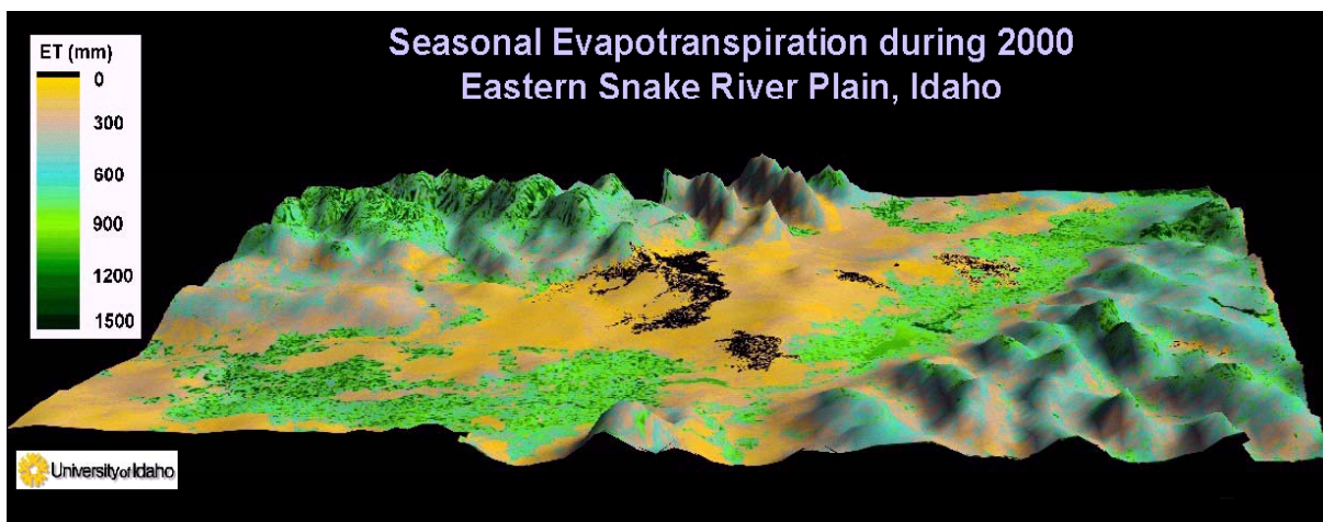
Figure 8. Evapotranspiration during the Growing Season for the ESRP area (300 km long region) in southern Idaho during March – October 2000.
