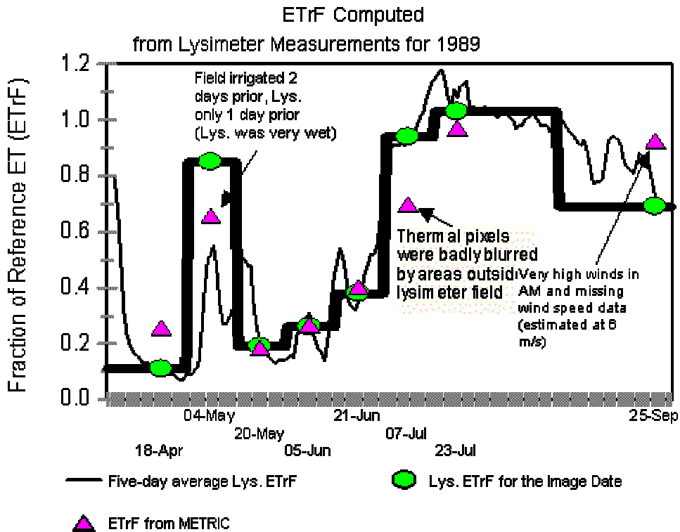
Figure 4. Results by METRIC and ET by Lysimeter as ET_{TF} (top). The thin line is the five-day average ET_{TF} for lysimeter and the thick line is the period average ET_{TF} method used to extrapolate between images (as compared to linear and curvilinear methods currently used).
