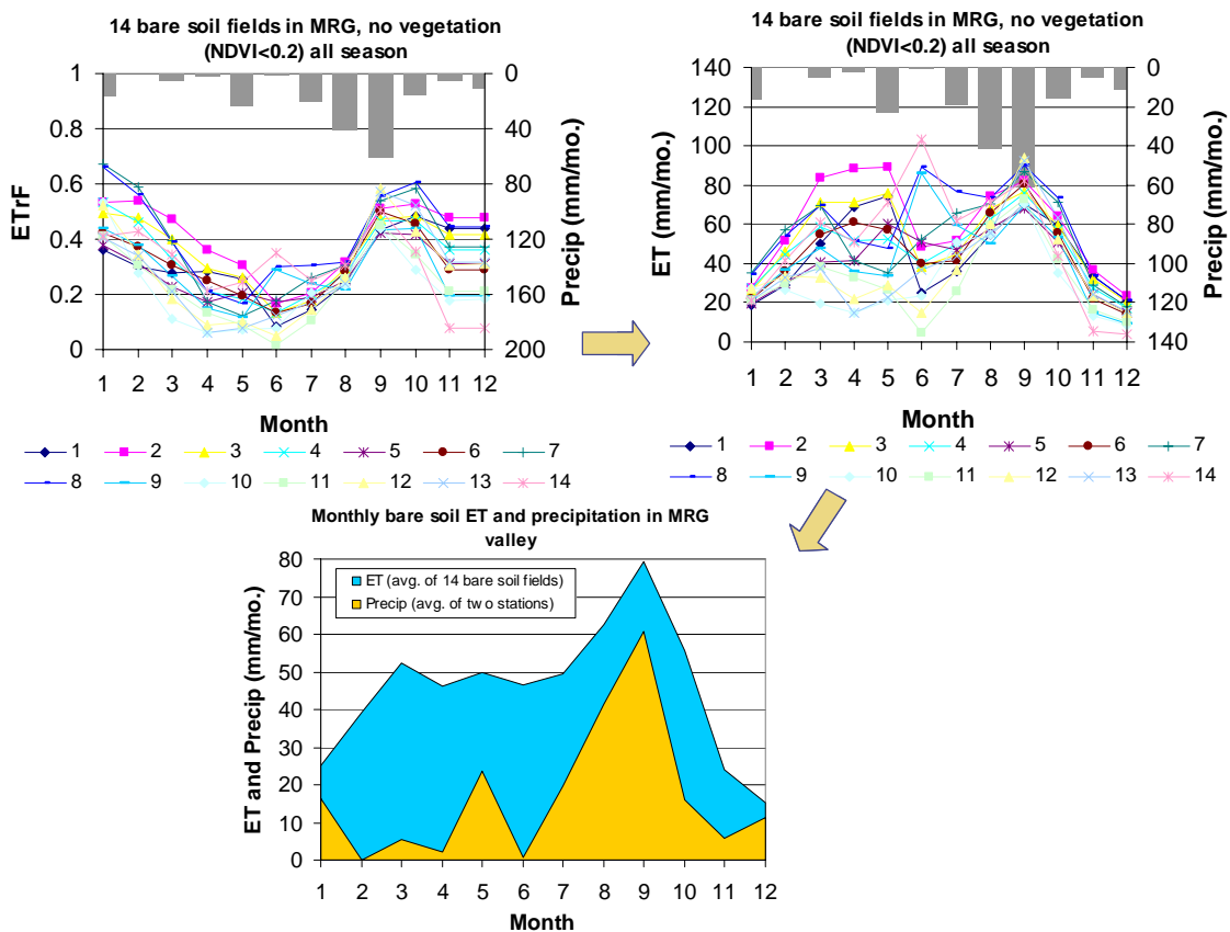
Figure 11. Evaporation during 2002 from continuously bare areas along the MRG and precipitation received at Angostura and Boys Ranch (averaged).
