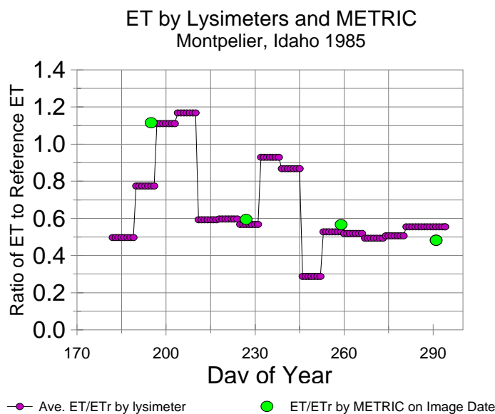
Figure 1. Comparison of ET_r fractions (i.e., K_c ) derived from 7-day lysimeter measurements near Montpelier, Idaho during 1985 and values from METRIC for four Landsat dates ( ET = \text{crop } ET and ET_r = \text{alfalfa reference } ET_r ).
