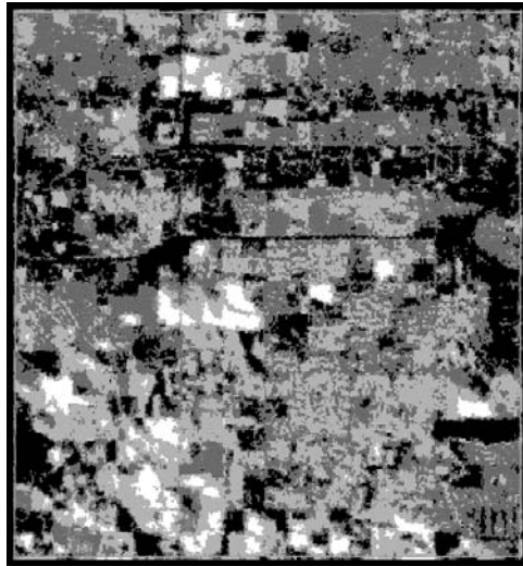
Figure 7. ET image of T3NR1E the Boise Valley (lighter intensity is higher ET)
