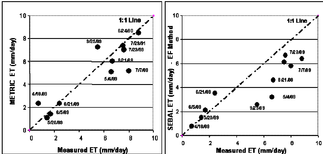
Figure 3. Comparison of daily ET from METRIC and ET_{TF} (left) and from SEBAL (version 2000) using EF (right) on satellite image dates for sugar beets (1989), potatoes (1988), peas (1990) and alfalfa (1991) (from Trezza, 2002).
